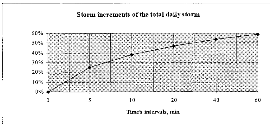
Figure 2. Twenty-five year frequency storm increment in Lithuania
