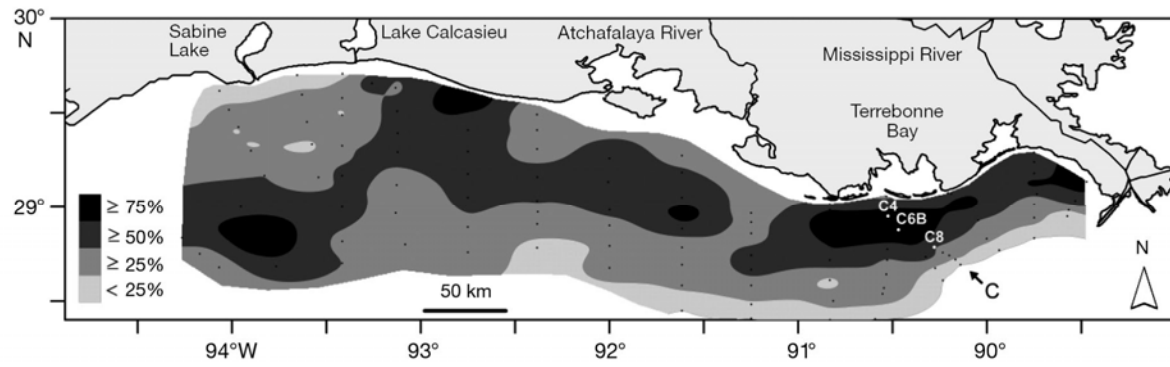
Figure 2. Frequency of mid-summer bottom-water hypoxia ( \leq 2 mg O 2 l -1 ) off the coast of Louisiana and Texas for 60 to 80 stations (small dots) sampled during the summer from 1985 to 2008.
